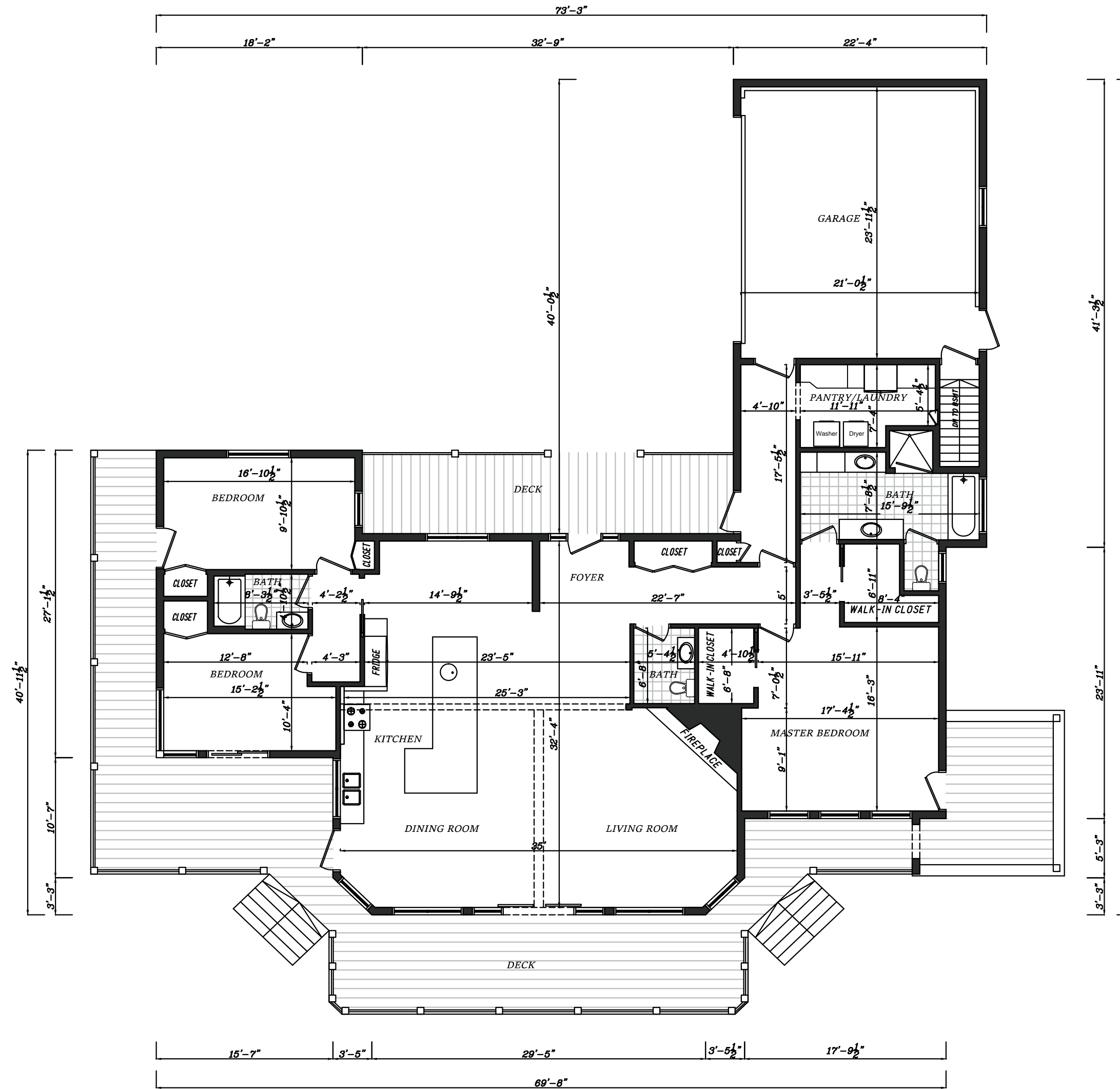
Main Level Floor Plan 46 Shore Road Lunenburg, NS
